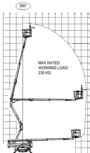
JLG-Modell X20J Plus
